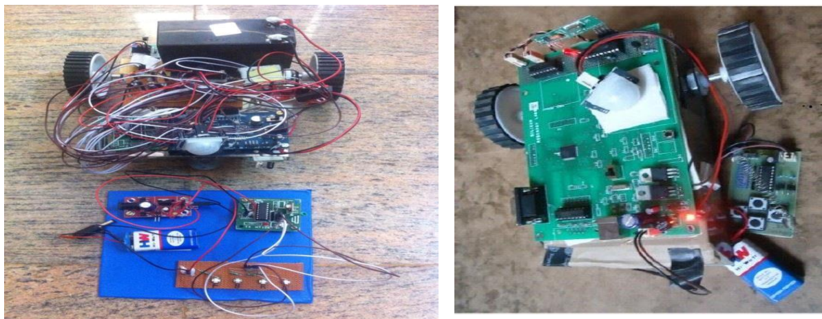
Figure 2: The Prototype of the proposed system
